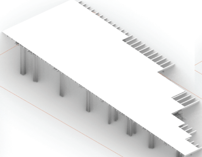
5 - Wood formwork roof
