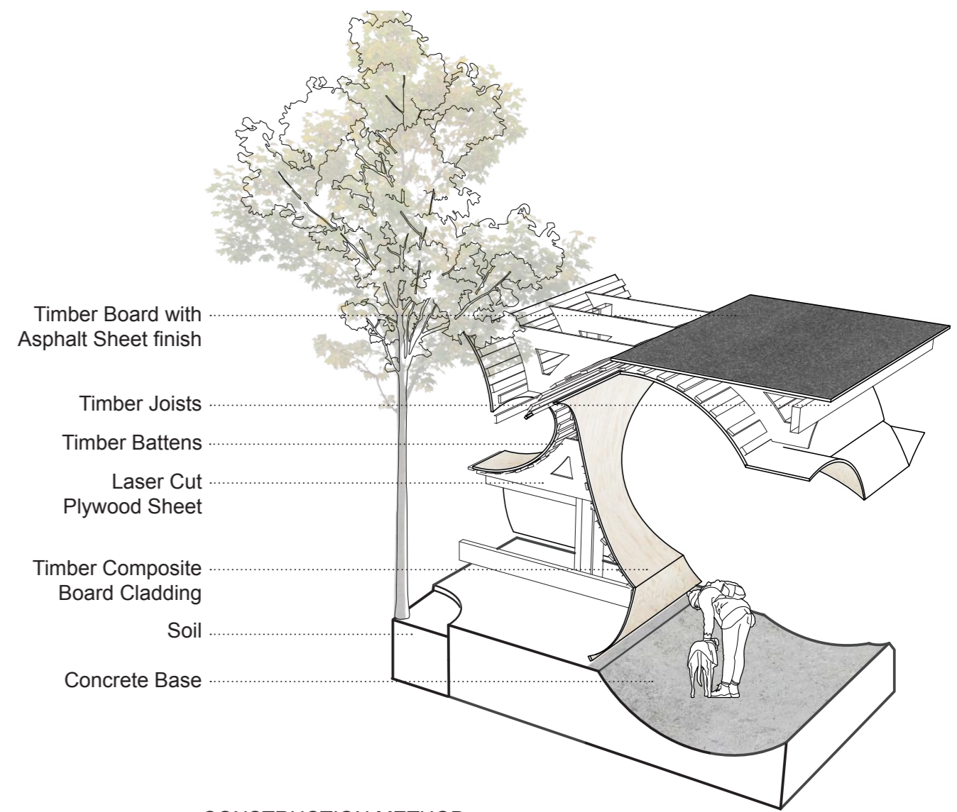
CONSTRUCTION METHOD
